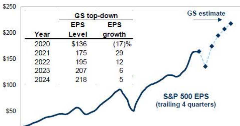
Exhibit 3: GS top-down S&P 500 EPS estimates as of November 12, 2020
