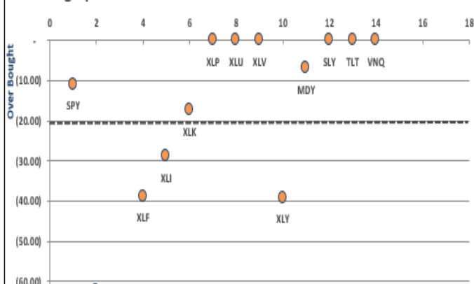
Overbought/Oversold 14-Periods
